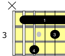
Bm7
