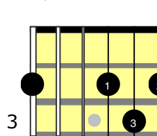
D/F#
