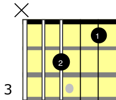
Am7
