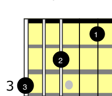
Am7/G
