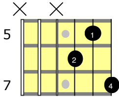
A (add9)
